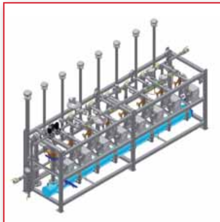
3D modeling of Gas Train
