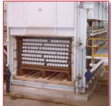
Homogenising Furnace
